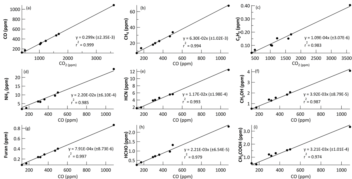
Figure 1. ER plots from plume N for (a) carbon monoxide, (b) methane, (c) acetylene, (d) ammonia, (e) HCN, (f) methanol, (g) furan, (h) formaldehyde, and (i) acetic acid measured by FTIR.
