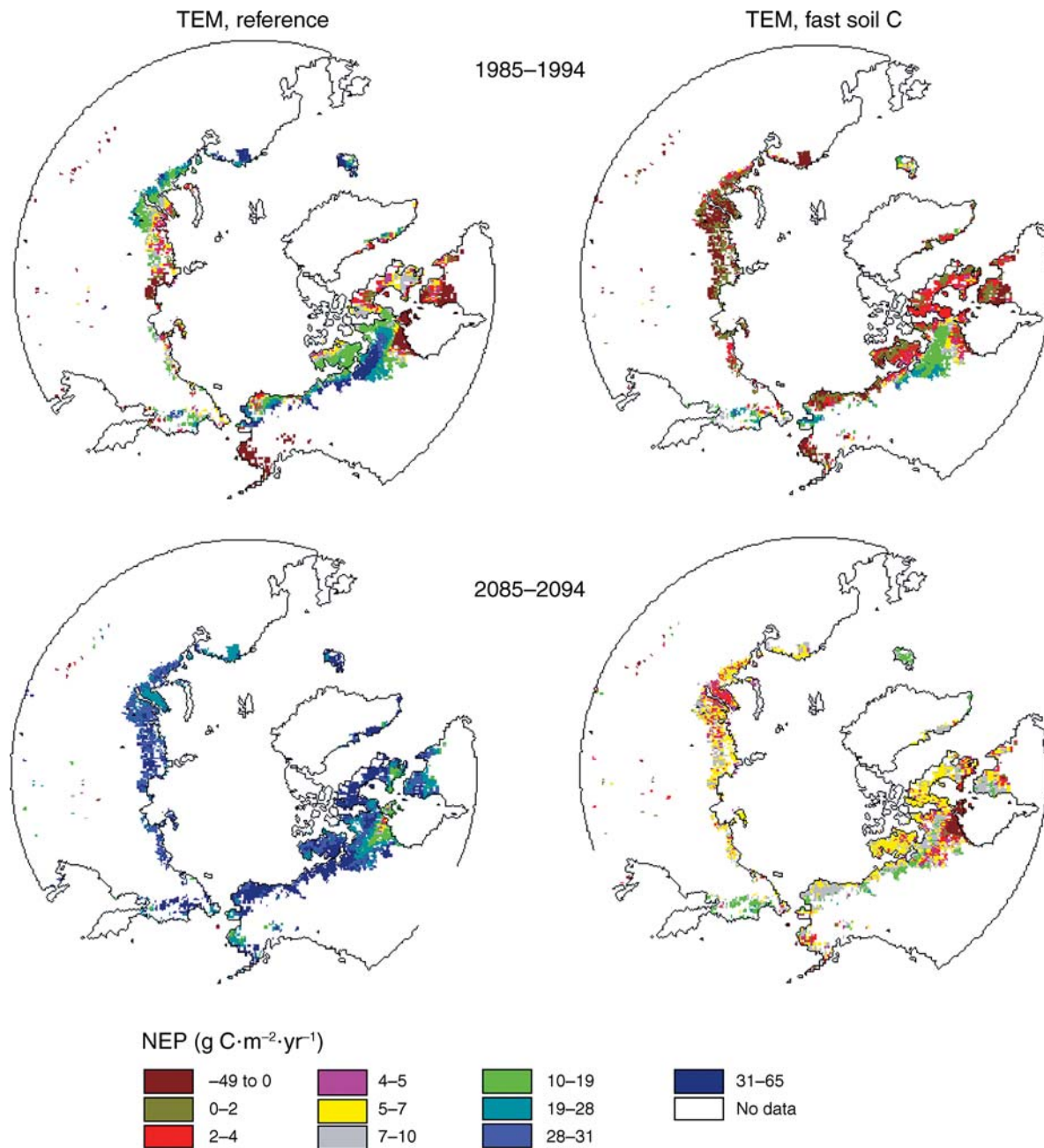
FIG. 6. Simulated spatial and temporal variability in mean annual NEP in moist tundra ecosystems north of 50^{\circ} N for the decades from 1985 to 1994 and from 2085 to 2094 as simulated by the Terrestrial Ecosystem Model (TEM) with the reference parameterization and by TEM for fast soil C dynamics (i.e., with much faster soil carbon turnover in comparison with the reference parameterization; Fig. 10 of Clein et al. 2000).
