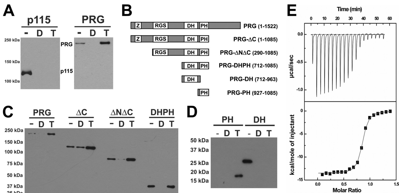
FIGURE 1. The PH domain from PRG interacts directly with activated RhoA. A , purified p115RhoGEF and PRG (12 pmol) were incubated with 80 pmol of immobilized GST-RhoA with no additional guanine nucleotide (–), 10 \mu M GDP ( D ), or 10 \mu M GTP \gamma S ( T ), as described under “Experimental Procedures.” RhoGEFs bound to the resin were subjected to SDS-PAGE and visualized by immunoblotting using anti-His 6 monoclonal antibody. B , schematic representation of truncated forms of PRG; included amino acids are listed at the right. PDZ domains are designated Z, C, or PH. C , purified PRG (full length or fragments as described in B ) were incubated with immobilized GST-RhoA, and RhoGEFs bound to the resin were analyzed by immunoblotting as described in A . D , purified PRG-DH and PRG-PH domains were incubated with immobilized GST-RhoA, with either no additional guanine nucleotide (–) or 10 \mu M GDP ( D ) or with immobilized GST-RhoA preloaded with GTP \gamma S ( T ). DH or PH domains bound to the resin were analyzed by immunoblotting as described in A . E , ITC profile for the binding of PRG-PH to RhoA·GTP \gamma S. Non-linear least squares fit using a “one set of sites” model resulted in the fit shown (solid line) at the bottom.
