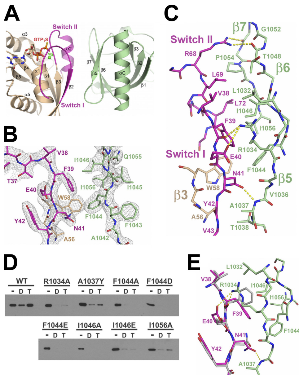
FIGURE 3. The PH-RhoA interface. A , ribbon diagram showing the interface between the PRG-PH domain and RhoA-GTP \gamma S using the same color scheme as in Fig. 2 A . B , electron density at the PH-RhoA interface. Electron density (cages) from a 2.7 Å \sigma_A -weighted 2F_o - F_c difference map (46) is contoured at 1.6 standard deviations above the mean. Residue labels are color-coded as shown in A . C , extensive contacts between switch regions of RhoA and the \beta 5- \beta 6- \beta 7 strands of the PH domain. Hydrogen bonds are drawn as dotted lines and colored yellow. Residues are labeled and color-coded as shown in A . D , purified PRG-DH-PH, wild-type (WT), or mutant were incubated with immobilized GST-RhoA, with no additional guanine nucleotide (–), 10 \mu M GDP (D), or 10 \mu M GTP \gamma S (T). DH-PH domains bound to the resin were analyzed by immunoblotting as described in the legend for Fig. 1. Mutations at the predicted RhoA binding site on PH had little effect on binding of PRG-DH-PH to nucleotide-free RhoA but severely impaired the ability of PRG-DH-PH to bind activated RhoA. E , structural comparison of switch I regions in RhoA-GTP \gamma S at the PH-RhoA interface. Elements from RhoA-GTP \gamma S in a complex with DH-PH are colored purple. Elements from RhoA-GTP \gamma S alone are colored gray. PH is colored green. Hydrogen bonds between RhoA-GTP \gamma S and the PH domain are drawn as dotted lines and colored yellow. The side chain conformations of Phe-39, Glu-40, and Asn-41 in switch I of RhoA change significantly upon binding to PH.
