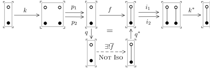
Figure 3.1: A counterexample to the (Strong) Fundamental Morphism Theorem in SiGrphs , SiStGrphs , and SiLiGrphs
