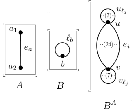
Figure 2.6: Pictures of the graphs for the counterexample to categorical “exponentiation with evaluation” in Grphs .
