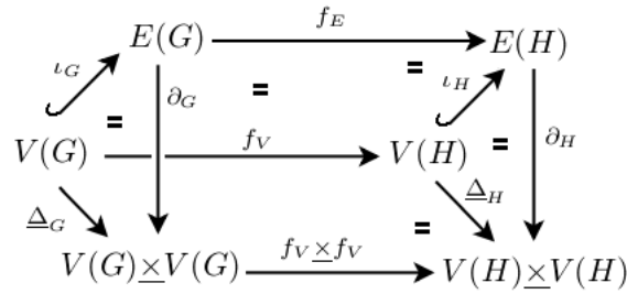
Figure 1.5: The Graph Morphism
