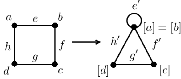
Figure 2.2: Example of a Quotient Graph in \mathcal{S}iStGr\mathcal{A}PHS
