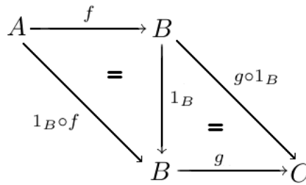
Figure 1.7: The Identity Law
