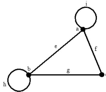
Figure 1.3: An Example of a Simple Graph
