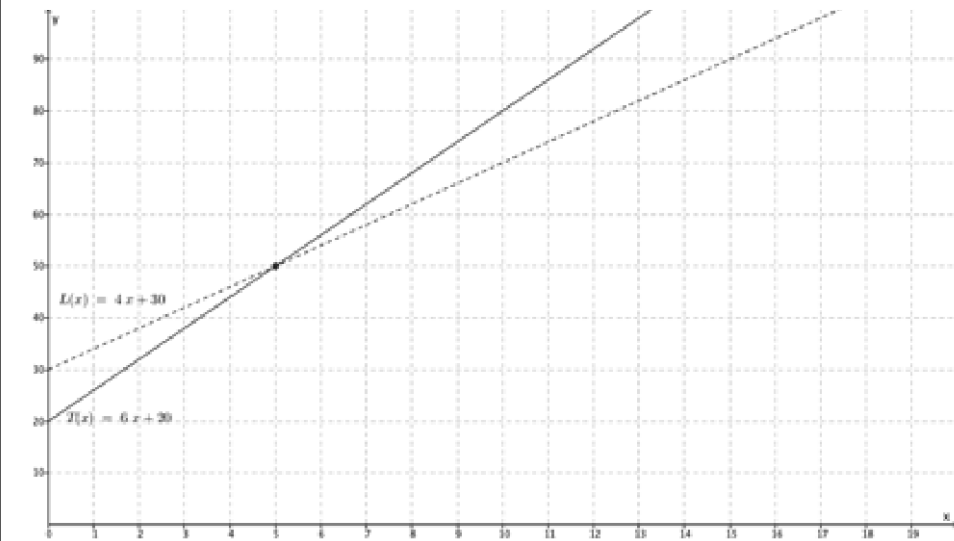
Figure 1 An example of a problem represented as two functions and as an equation
